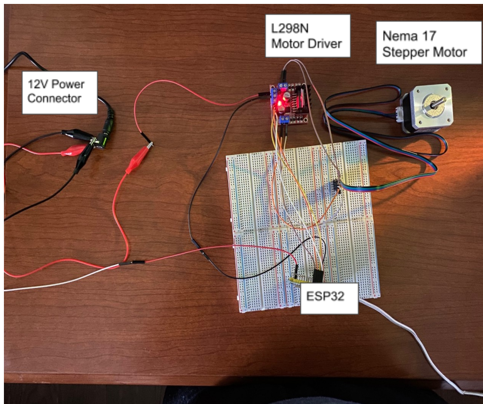
Figure 47 - Motor System Breadboard Test
