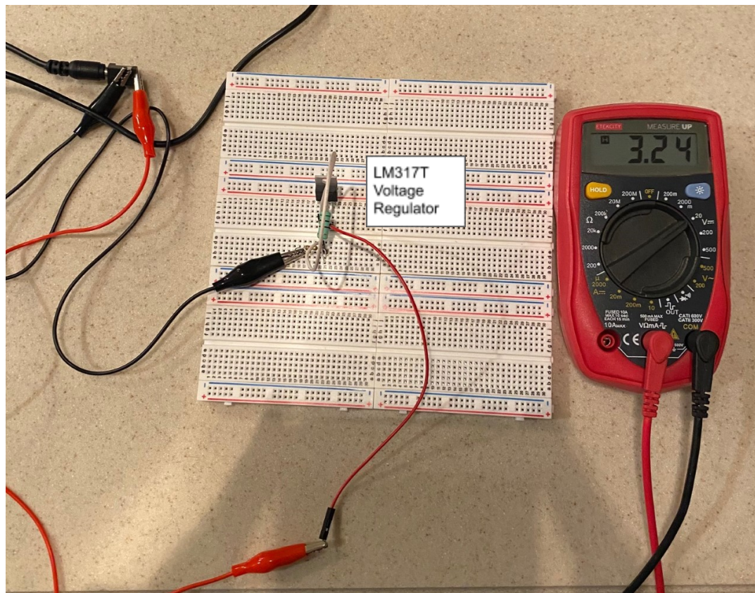
Figure 40 - 3.3V Voltage Regulator Breadboard Test
