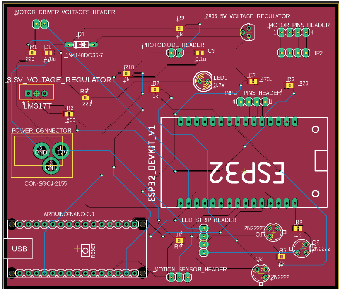
Figure 55 - PCB Layout in Eagle
