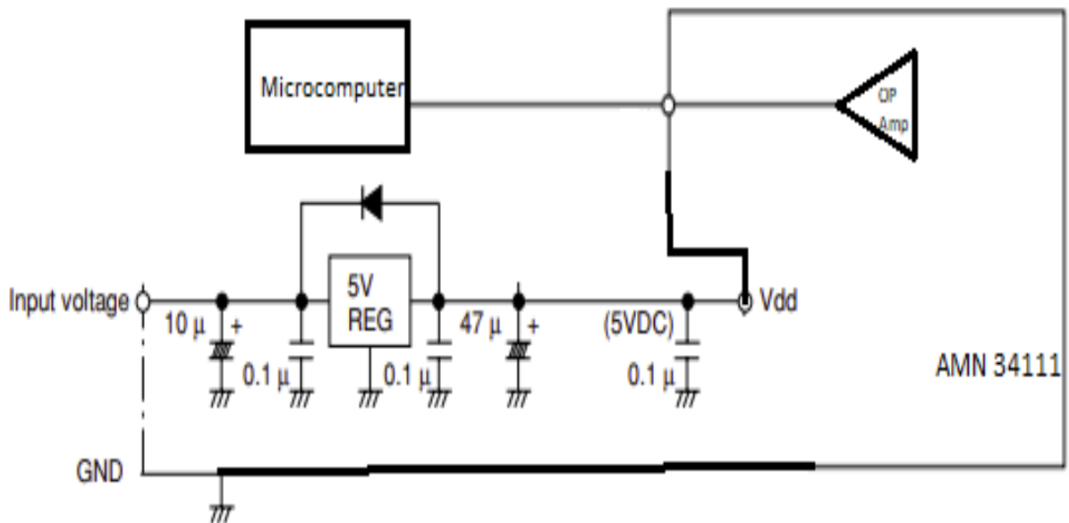
Figure 53 - Alliedelect AMN 34111 analog circuit (Panasonic recommendation circuit)
