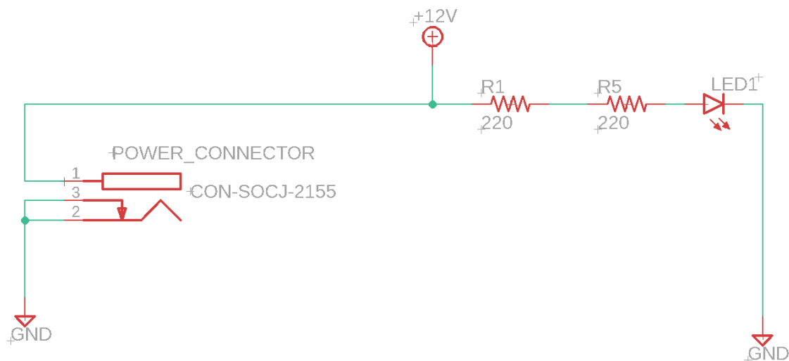
Figure 41 - Power Connector Circuit Schematic
