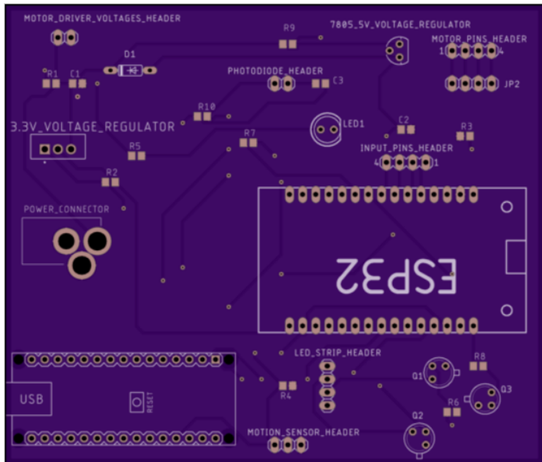
Figure 56 - PCB Board Prototype
