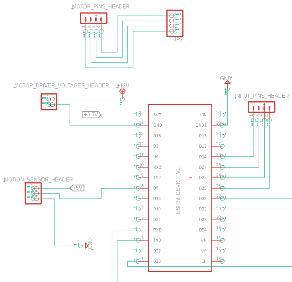
Figure 48 - Motor System Circuit Schematic
