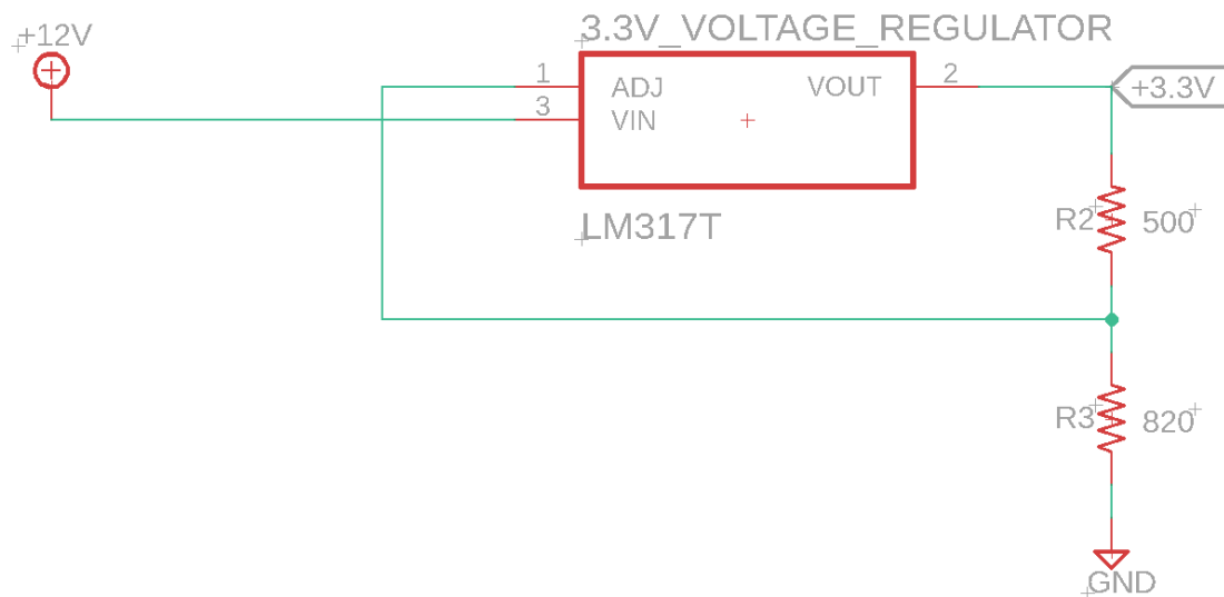
Figure 39 - 3.3V Adjustable Voltage Regulator Schematic
