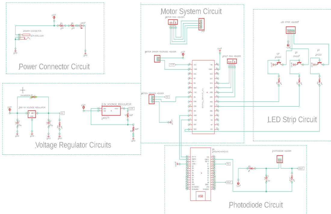
Figure 54 - Final PCB Schematic
