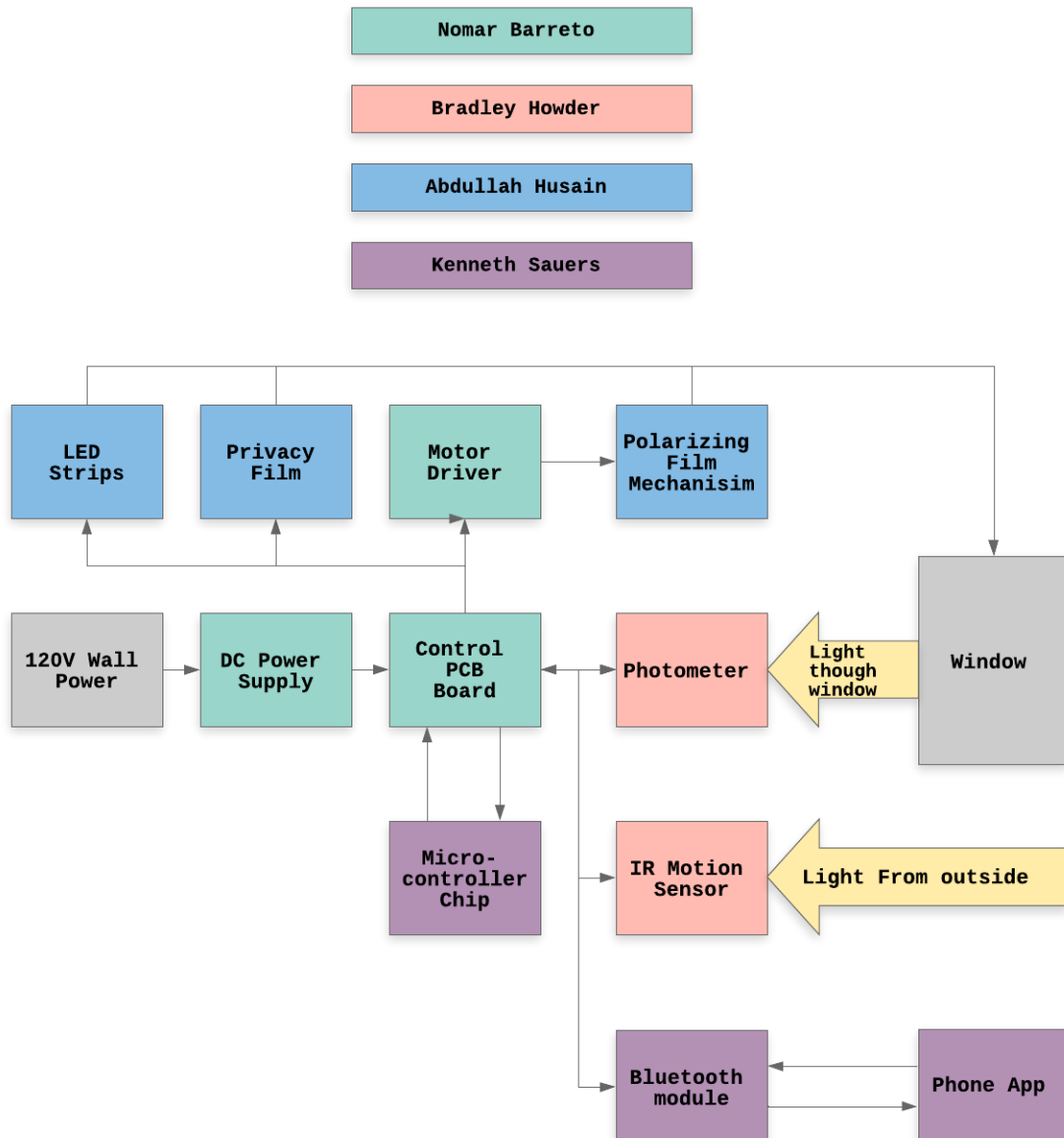
Figure 2 - Block diagram
