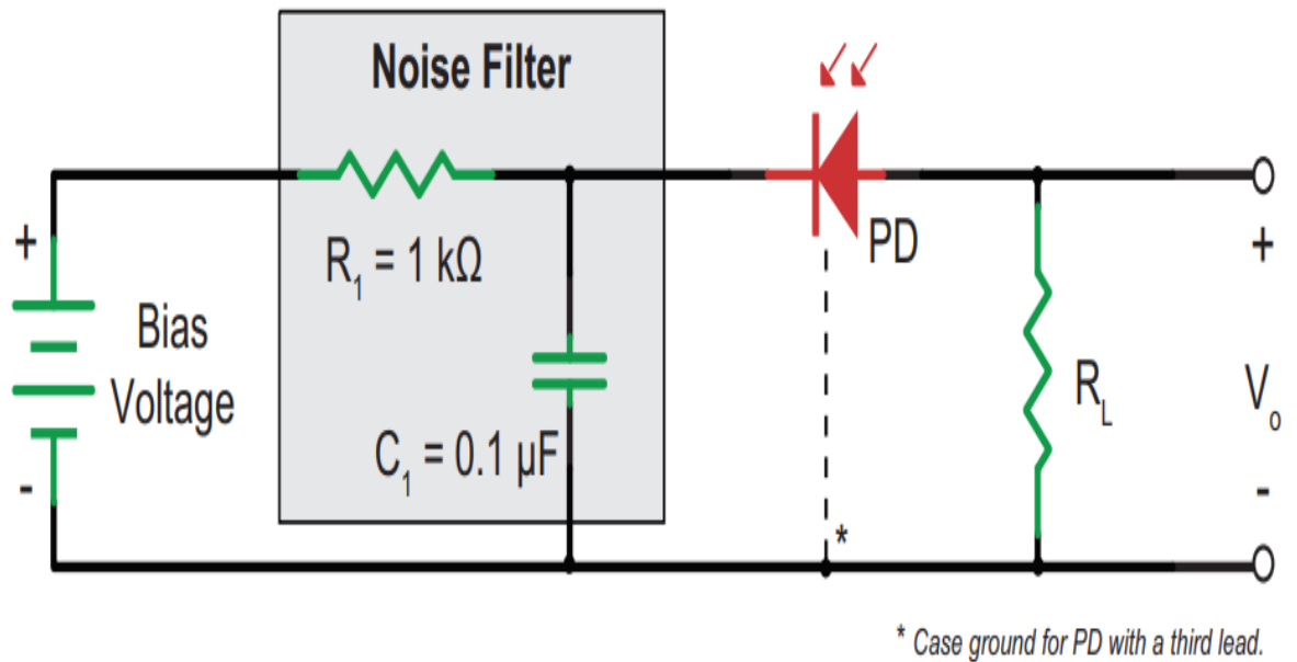
Figure 51 - Photodiode FDS1010 circuit diagram (Thorlabs circuit diagram)
