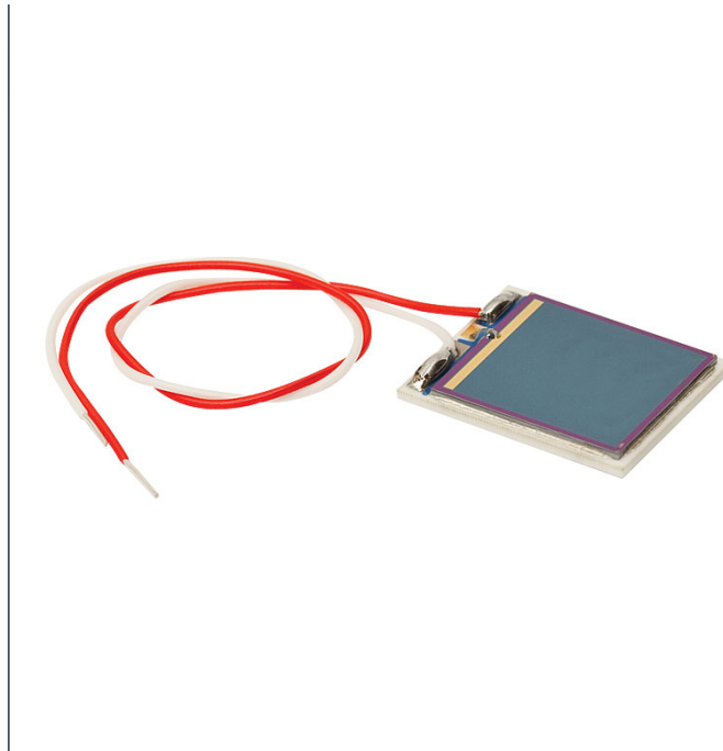
Figure 26 - Thorlabs FDS1010
