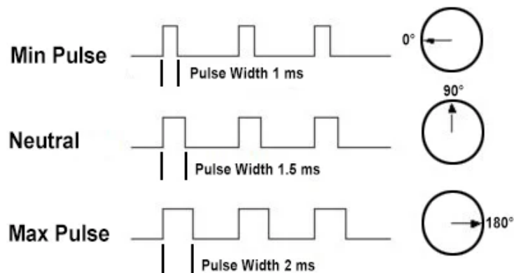
Figure 8 - Pulse Width Modulation (PWM) effect on Servo Motor Rotation Angle Image Taken from (jameco.com)
